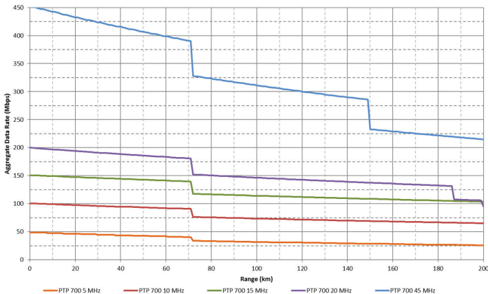
Aggregate Data Rate PTP 700 Unrestricted for Line of Sight paths
