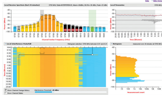
Spectrum Management - Radar Avoidance with Dynamic Spectrum Optimization
