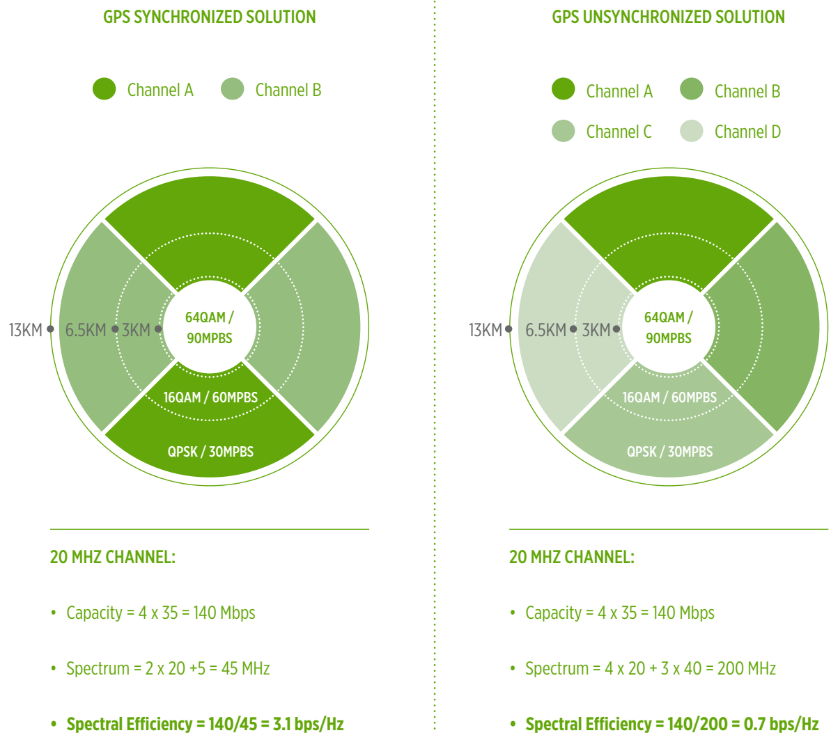
Figure 4: Spectral Efficiency Comparison
