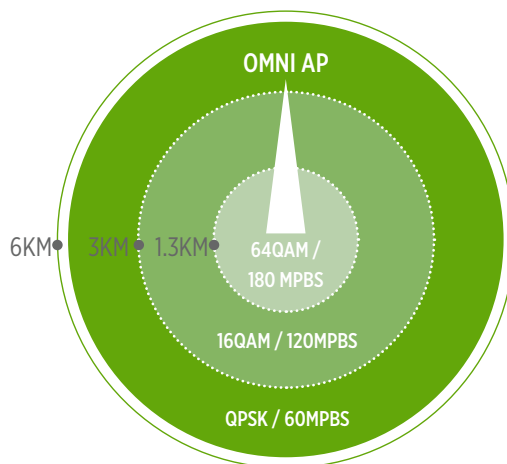
Figure 5: Omni Access Point with 40 MHz Channel
