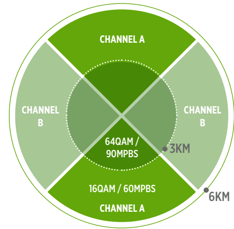
Figure 7: Sector Access Point with 20 MHz Channels
