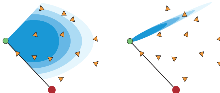
Figure 5 - Example of uplink throughput and interference rejection improvement
