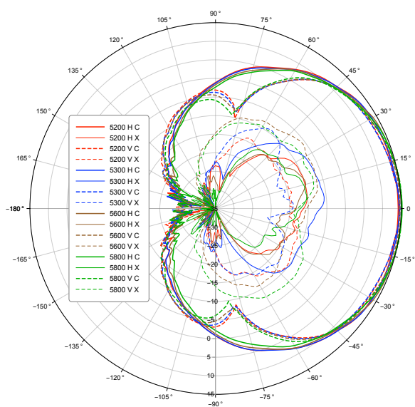
5 GHz Azimuth
