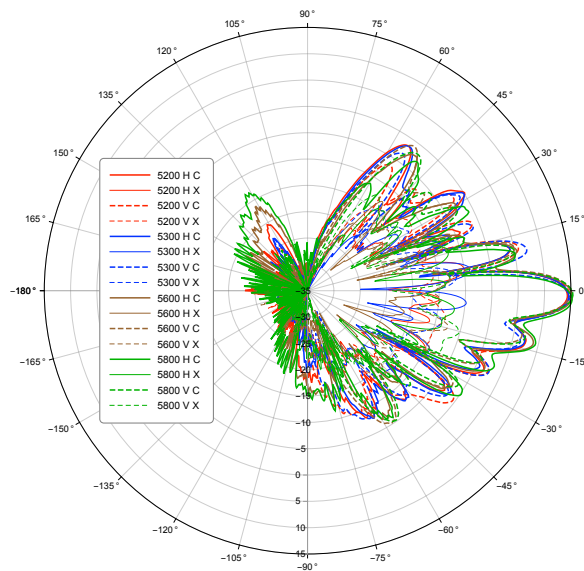
5 GHz Elevation
