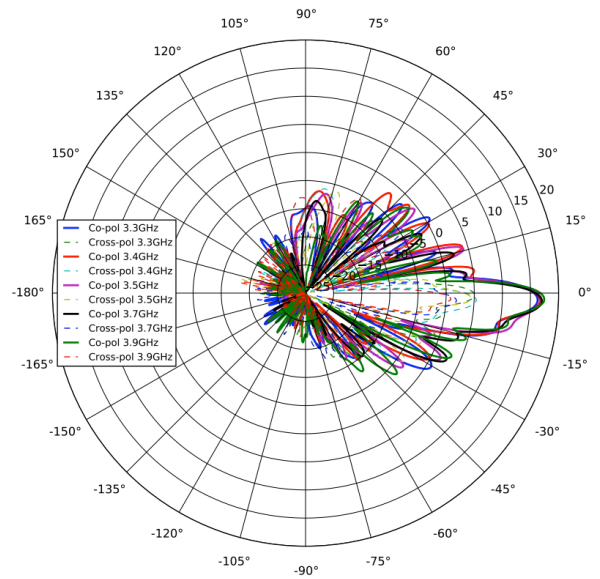
3 GHz Elevation
