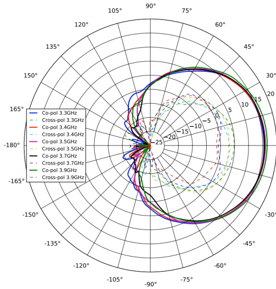
3 GHz Azimuth
