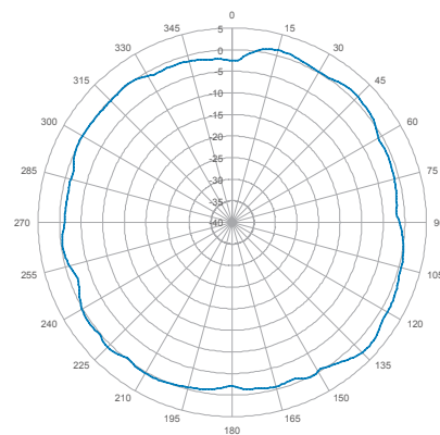
5 GHz Elevation
