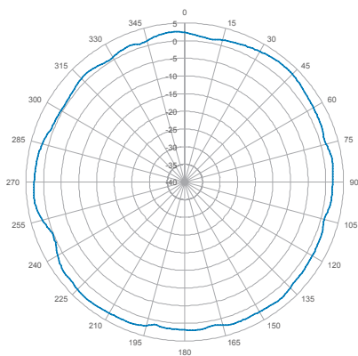
5 GHz Azimuth
