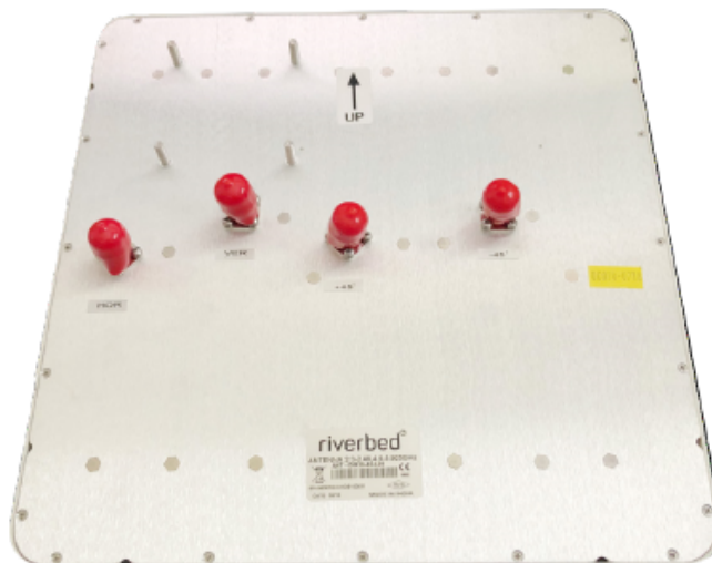
Antenna/Connectors
