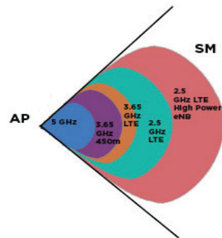
Figure 5 – Covering Hard to Reach CAF Phase II SMS with 450m in 3.65 GHz and cnRanger (LTE)
