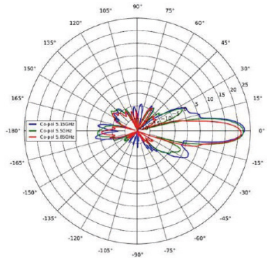
Elevation, Vertical
