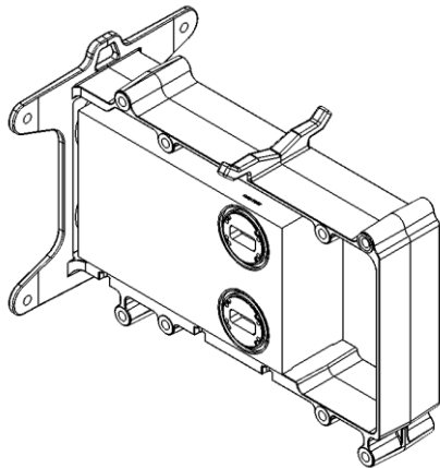
Figure 9 Dual Coupler/Splitter/Circulator
