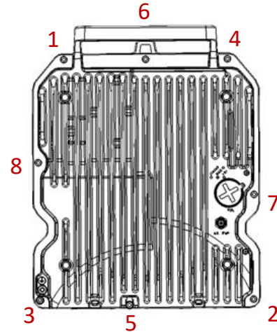
Figure 50 Order of Fastening Screws
