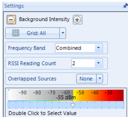
Figure 21. Additional Global Settings in Analyze Mode
