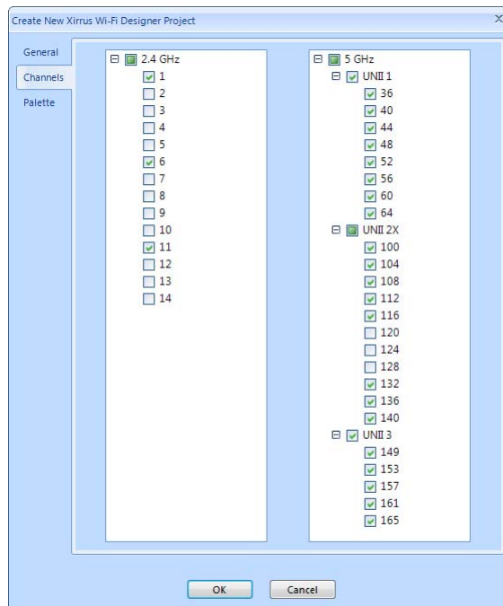
Figure 33. Channel Selection Options
