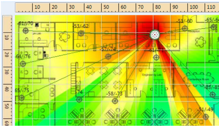
Figure 20. Interpolated Heatmap
