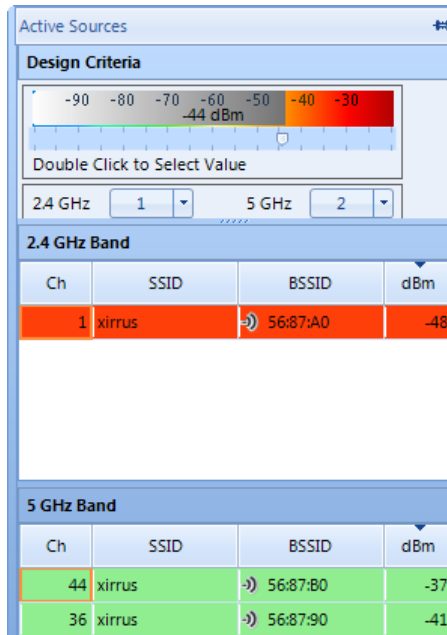
Figure 37. Active Sources Panel
