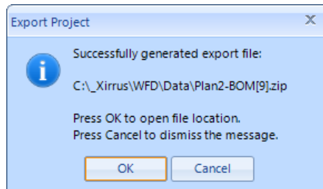
Figure 28. Export Complete
