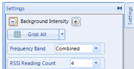
Figure 9. Settings Panel
