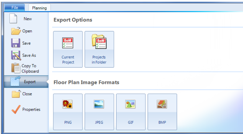
Figure 24. Export Options
